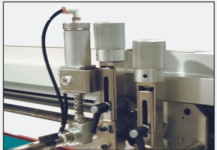
Pneumatic “Squeegeelizer” automatically adjusts for uniform squeegee pressure.
