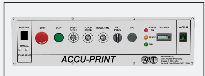
Operator-friendly control panel.
